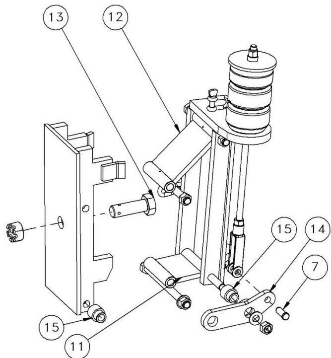
PENTURE DROITE 4-8-30 DEGRES 4-8-30 DEGREES RIGHT HINGE
