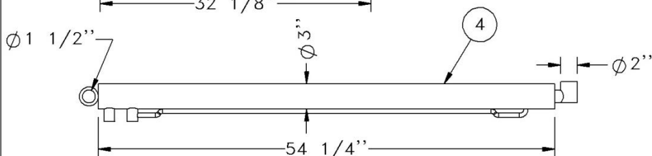
CYLINDRE COLONNE AVANT 48" 48" FRONT POST CYLINDER
