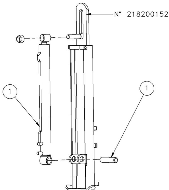
VUE A COLONNE AVANT HYDR. 26''VIEW VIEW A 26'' HYDR. FRONT POST
